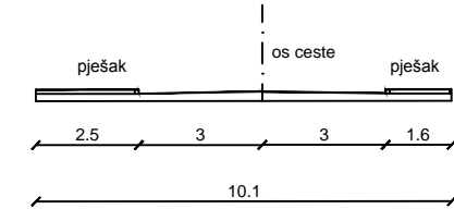
C1-C1
